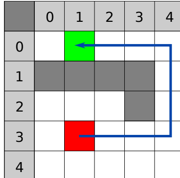
Figure 338: The path taken by the Dijkstra Algorithm
